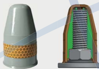
Bolt & Nut Protective Caps
